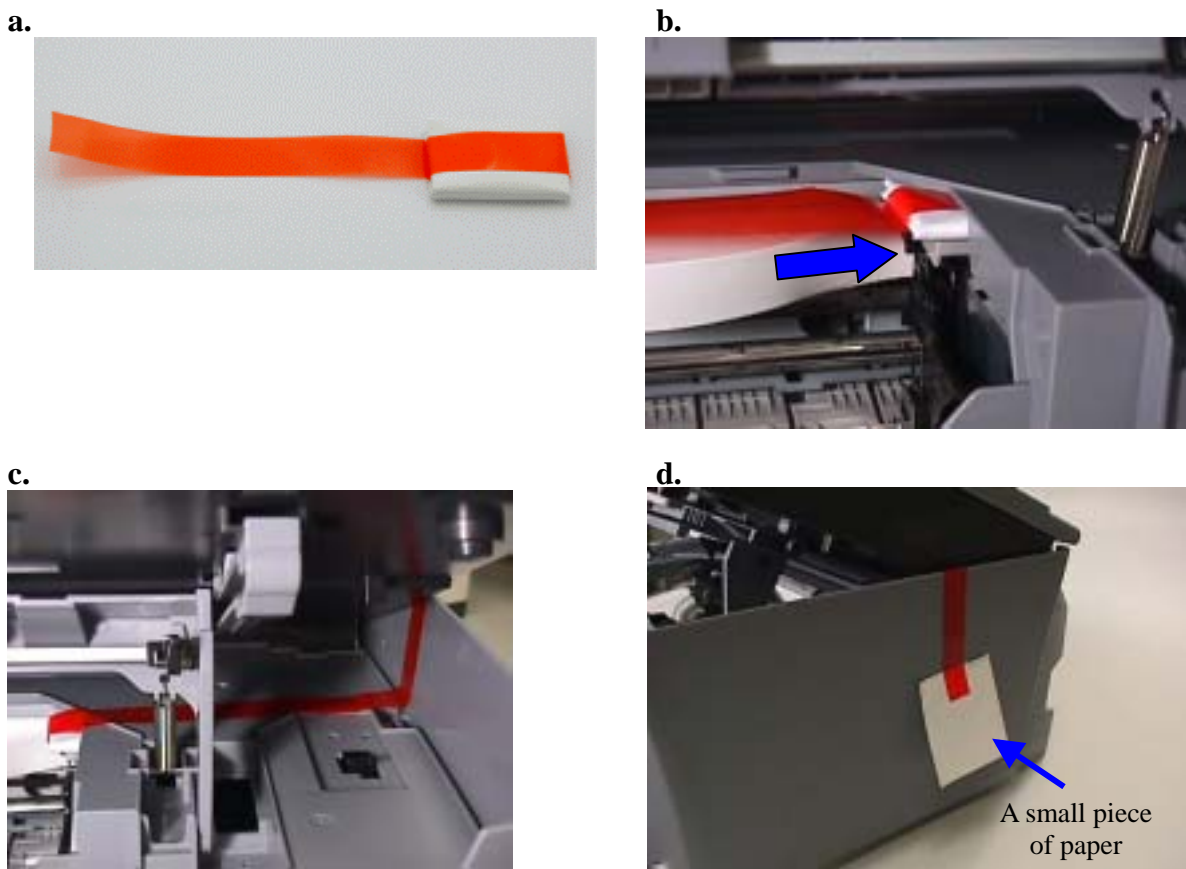
Figure 1-38 How to fix the Carriage
