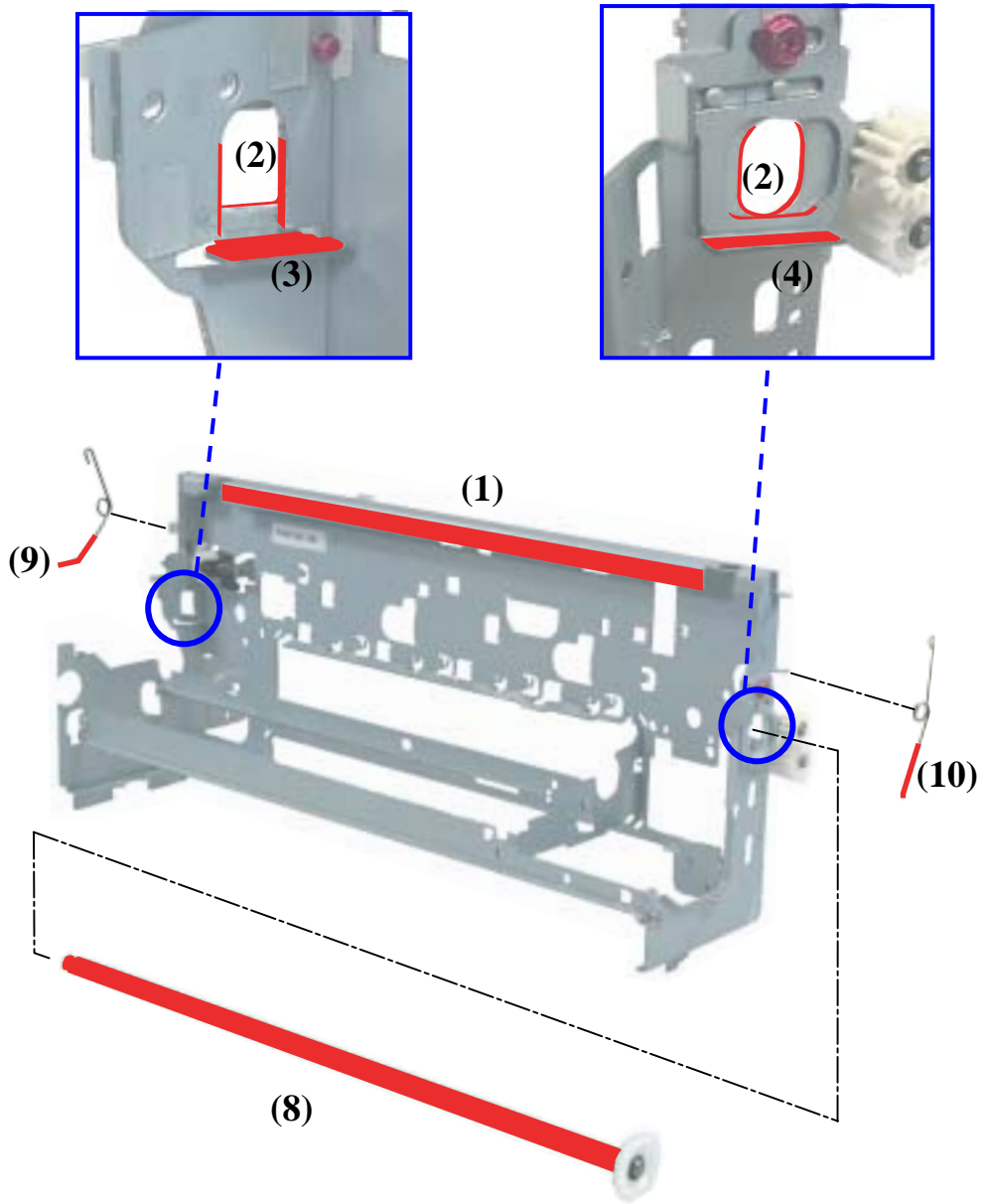
Figure 1-20 Grease application1
